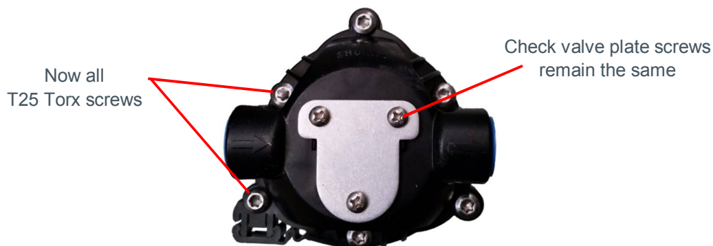
Fig 1. Example pump head with new screws
